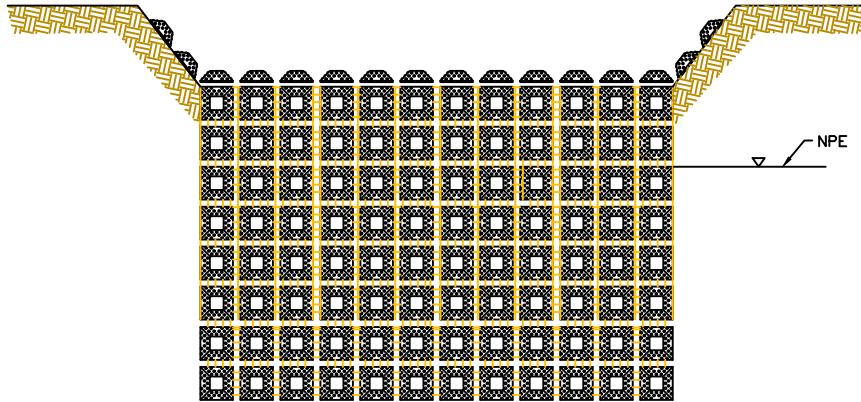
ELEVATION VIEW
